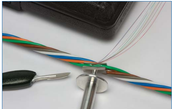
NFT-000 No-Slack Optical Fiber Access Tool (NOFAT) | Photo LAN1345
